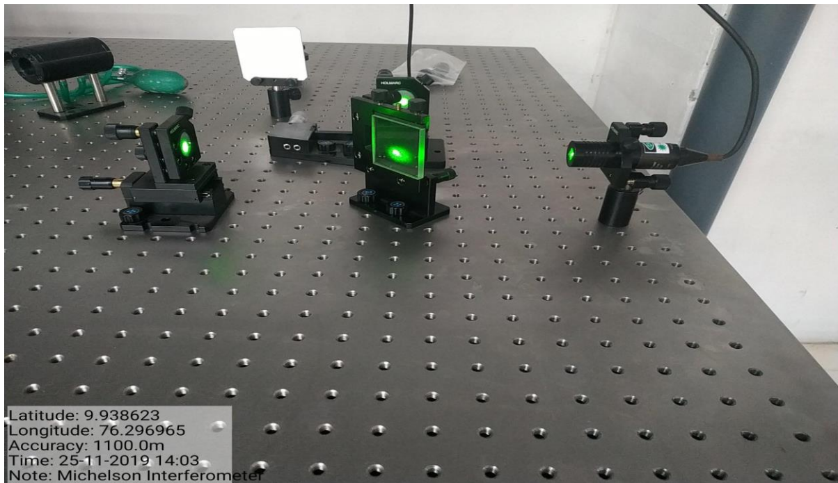
Michelson interferometer
