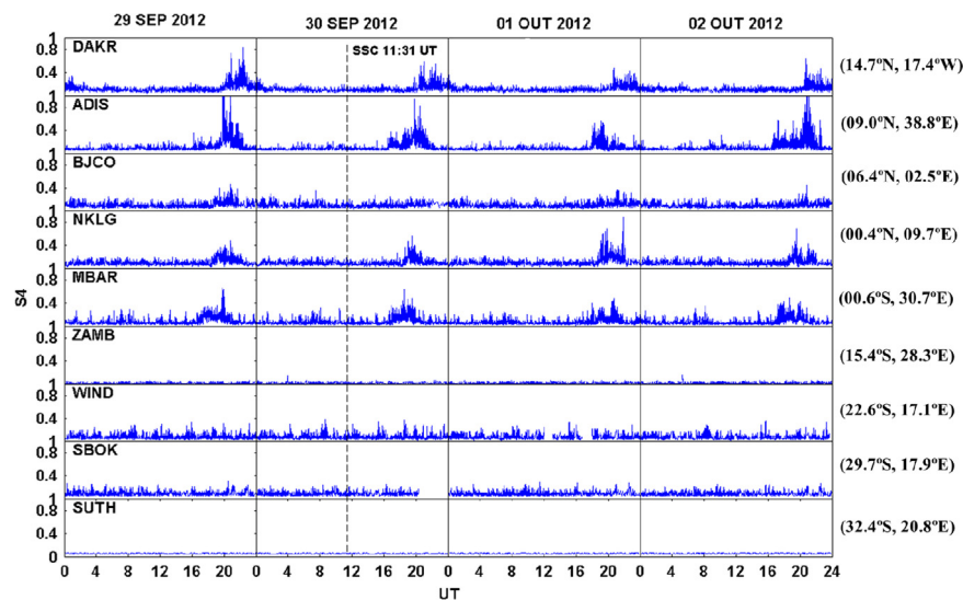
Fig. 8. GPS amplitude scintillations ( S_4 index) for the satellites with elevation angles higher than 30^\circ at 9 receiving stations at African Sector on the days 29, 30 September, 01 and 02 October 2012.
