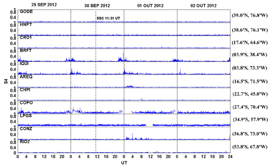
Fig. 7. GPS amplitude scintillations ( S_4 index) obtained from satellites (with elevation angles higher than 30^\circ ) at 11 receiving stations at American Sector during the period 29 September–02 October 2012.
