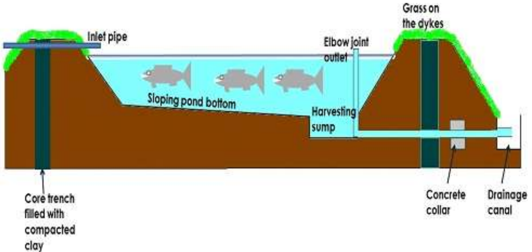
A cross section of a completed pond showing the position of various structures
